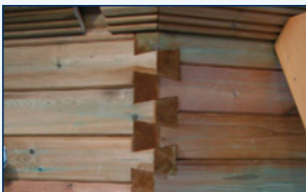
Wooden frame (45mm) in treated, grade 4 red Pinewood
